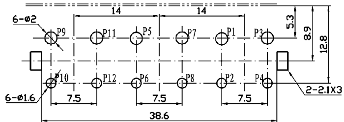
Dimensions of PC board holes (commend)
