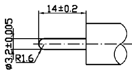
Gauge Plug
