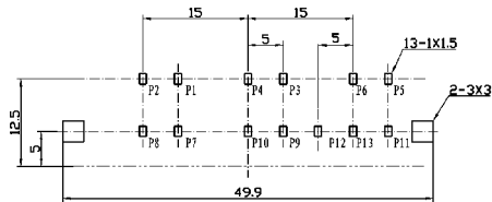
Dimensions of PC board holes (Commend) Top View (t=1.6mm) ⊗
