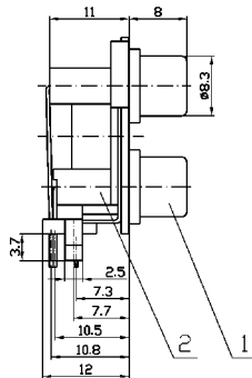
Gauge Plug
