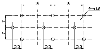
Dimensions of PC board holes (Commend)
