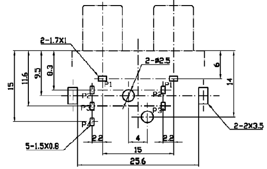
Dimensions of PC board holes (Commend) Bottom View (t=1.6mm) \odot
