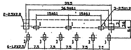
Dimensions of PC board hole
