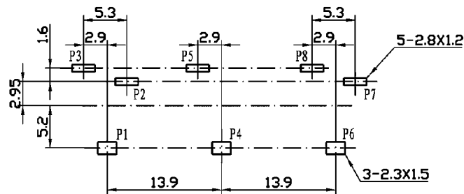
Dimensions of PC board holes (Commend)
