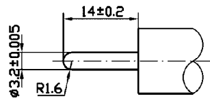
Gauge Plug
