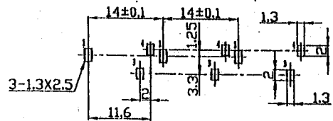
Dimensions of PC board holes Ⓞ
