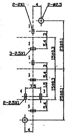
Dimensions of PC board holes
