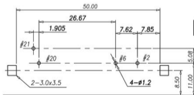
Recommend PCB Layout Jack Top View
