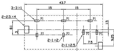
Dimensions of PC board holes (Commend) Bottom View ( t=1.6\text{mm} )
