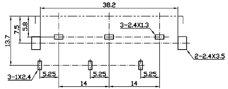
Dimensions of PC board holes (Commend) Bottom View (t=1.6mm) ⊙
