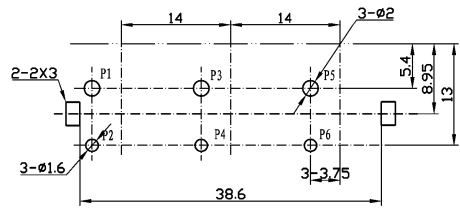
Dimensions of PC board holes (Commend) Bottom View (t=1.6mm) ⊙
