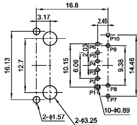
Recommend PCB Layout Jack Top View
