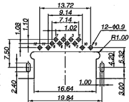
Recommend PCB Layout Jack Top View
