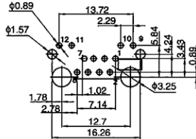
Recommend PCB Layout Jack Top View
