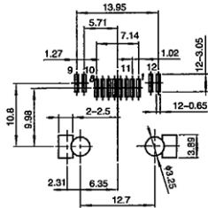
Recommend PCB Layout Jack Top View
