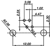
Recommend PCB Layout Jack Top View
