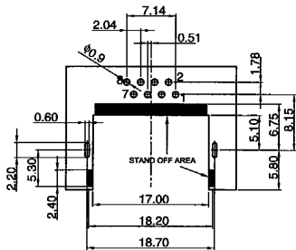
Recommend PCB Layout Jack Top View
