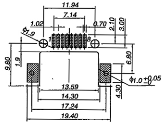
Recommend PCB Layout Jack Top View
