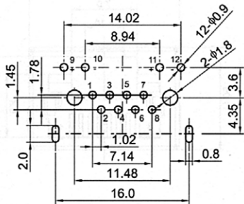
Recommend PCB Layout (Jack Top View) Tolerance: \pm 0.05\text{mm}
