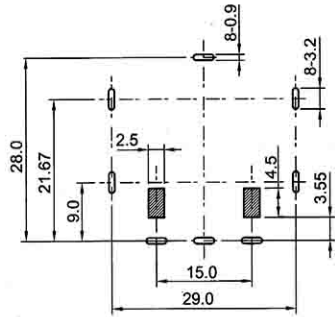
Recommend PCB Layout Jack Top View
