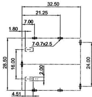
Recommend PCB Layout Jack Top View
