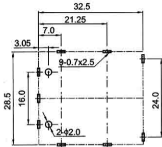
Recommend PCB Layout Jack Top View
