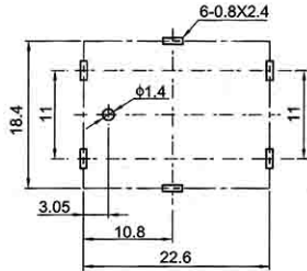
Recommend PCB Layout Jack Top View
