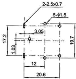
Recommend PCB Layout (Jack Top View)
