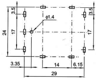
Recommend PCB Layout (Jack Top View)
