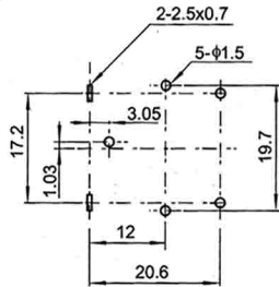
Recommend PCB Layout (Jack Top View)
