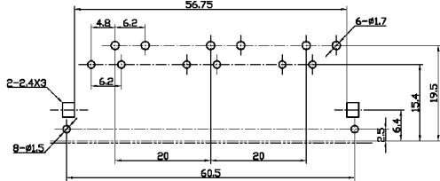
Dimensions of PC board holes (Comment)
