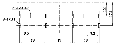
Dimensions of PC board holes (Commend)
