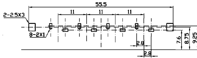
Dimensions of PC board holes (Commend)
