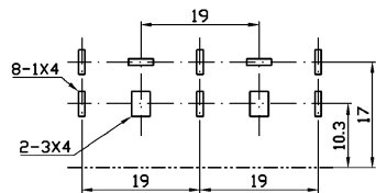
Dimensions of PC board holes (Commend)
