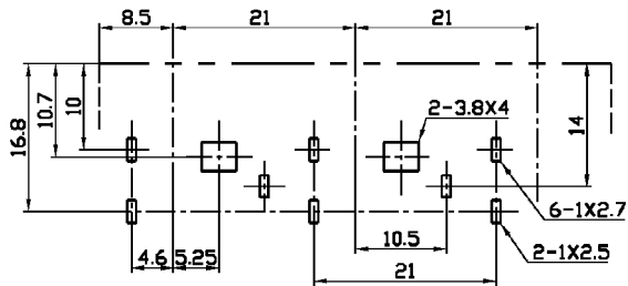
Dimensions of PC board holes(Commend)
