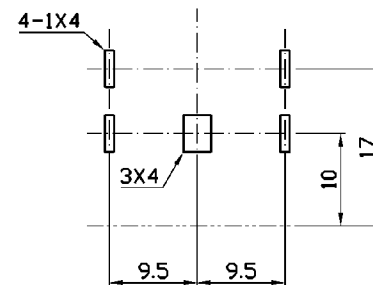
Dimensions of PC board holes
