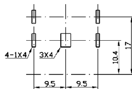
Dimensions of PC board holes (Commend)
