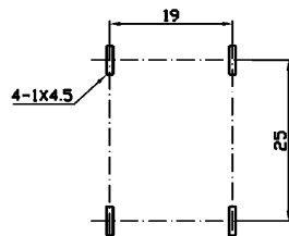
Dimensions of PC board holes
