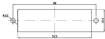
Dimensions of build in board hole(commend)
