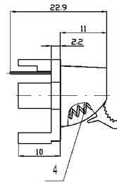
Dimensions of build in board hole(commend)
