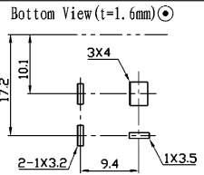
Dimensions of PC board holes (Comment)
