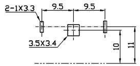
Dimensions of PC board holes (Commend) Top View (t=1.6mm) ⊗
