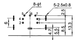
Recommend PCB Layout Jack Top View
