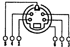
S Jack
