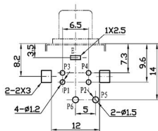
Dimensions of PC board holes (Commend)
