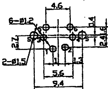
Dimensions of PCB board holes (Command)
