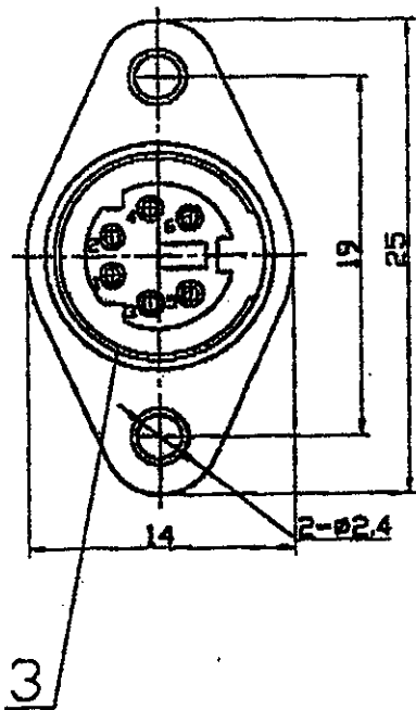
Dimensions of PCB board holes (Command)
