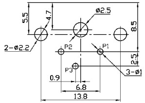
Dimensions of PC board holes (Comment) Bottom View \odot
