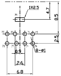
Dimensions of PC board holes (Comment)
