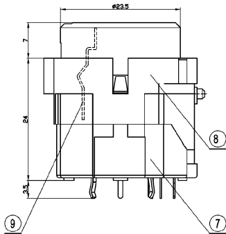
A向 View From A
