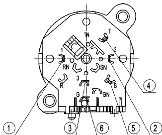
A向 View From A
