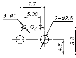
Recommend PCB Layout Jack Top View
