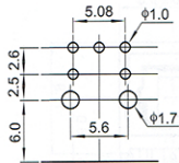
Recommend PCB Layout Jack Top View
