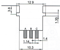
Recommend PCB Layout Jack Top View
